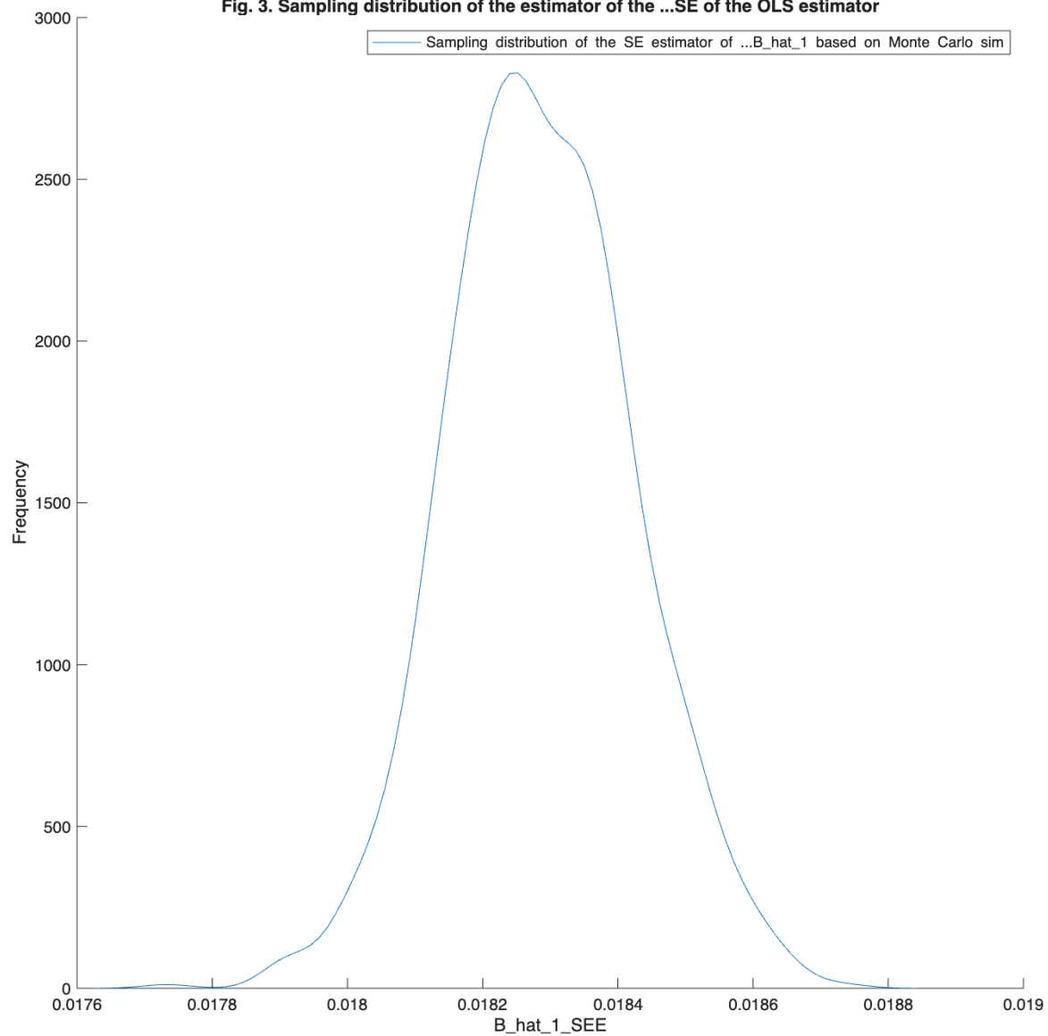
Fig. 3. Sampling distribution of the estimator of the ...SE of the OLS estimator
