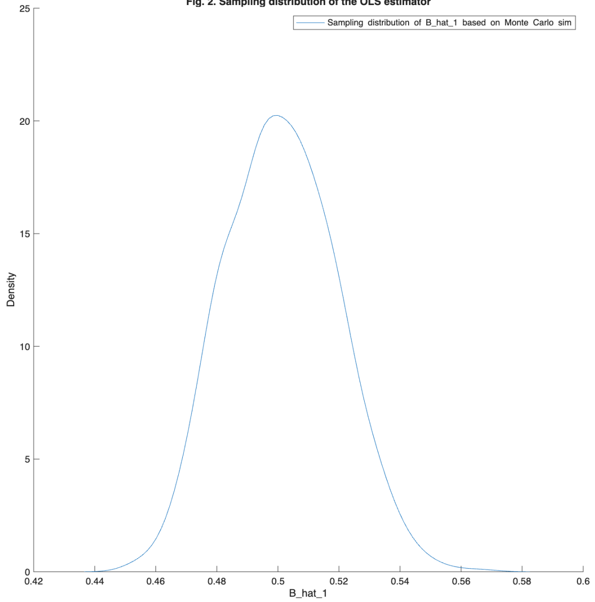
Fig. 2. Sampling distribution of the OLS estimator
